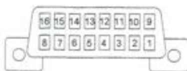
OBD-II Connector
